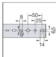
Perforation details DIN 43659 EN 50 085-2-3 width 25, 40 and 60 mm
